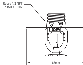
Shield com sprinkler mod F1FR56
